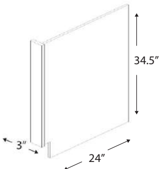
DISHWASHER RETURN PANEL
